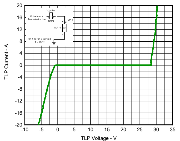
Fig 6. TLP Measurement
