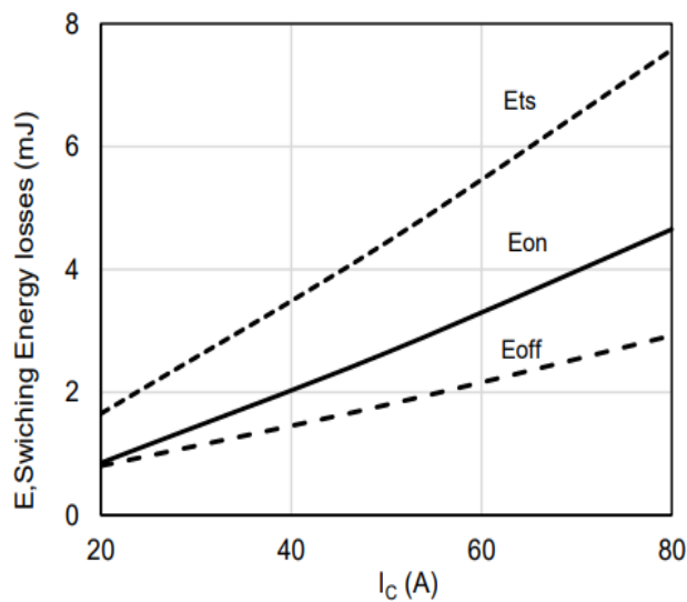
Fig 10. Switching Energy Loss vs. Collector Current
