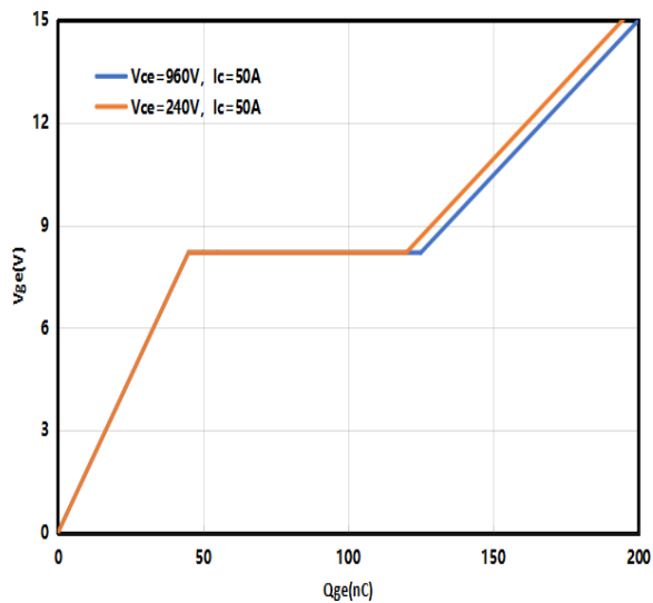
Fig 5. Gate Charge
