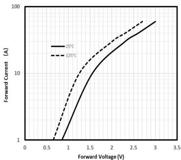
Fig 8. Typical Diode VF vs. IF Characteristic
