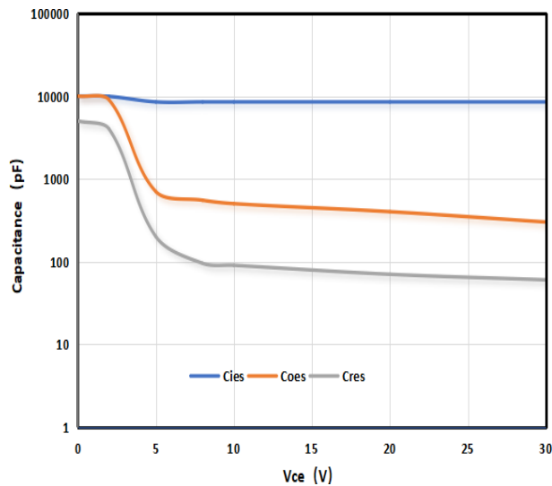
Fig 6. Typical Capacitance
