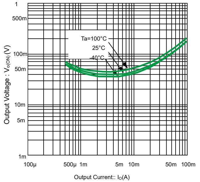
Fig 4.Output current vs. output voltage @Io/Ii=20
