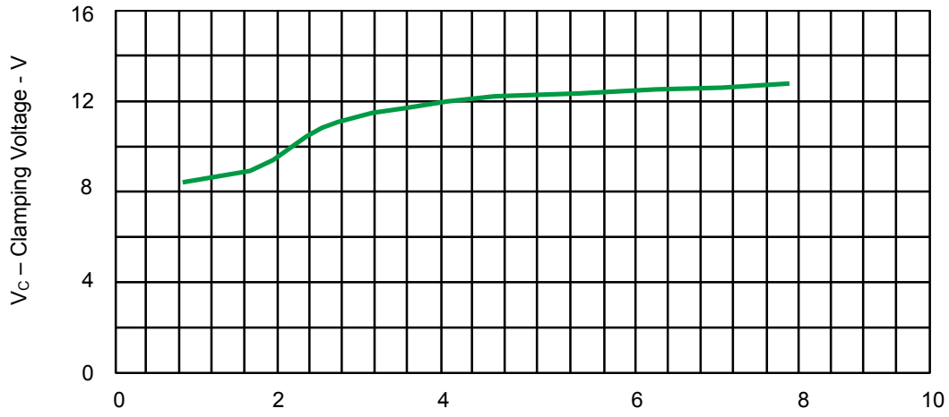
Fig.1 Typical Clamping Voltage VS Peak Pulse Current for PESDLC353T5VU
