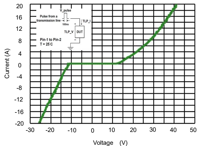
Fig 6. TLP Measurement
