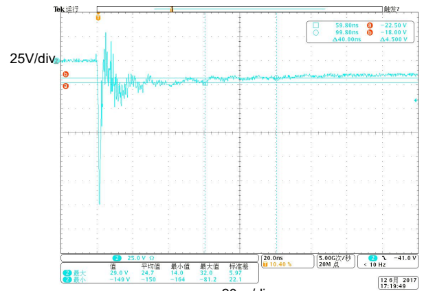
20ns/div Fig 8. ESD clamping voltage (IEC61000-4-2 -8KV contact)
