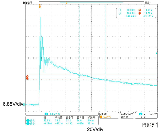
Fig 8. ESD clamping voltage (IEC61000-4-2 +8KV contact)
