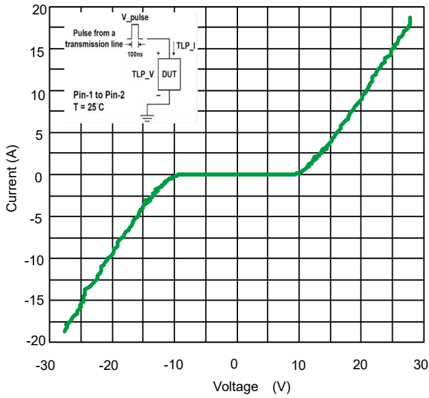
Fig 7. TLP Measurement
