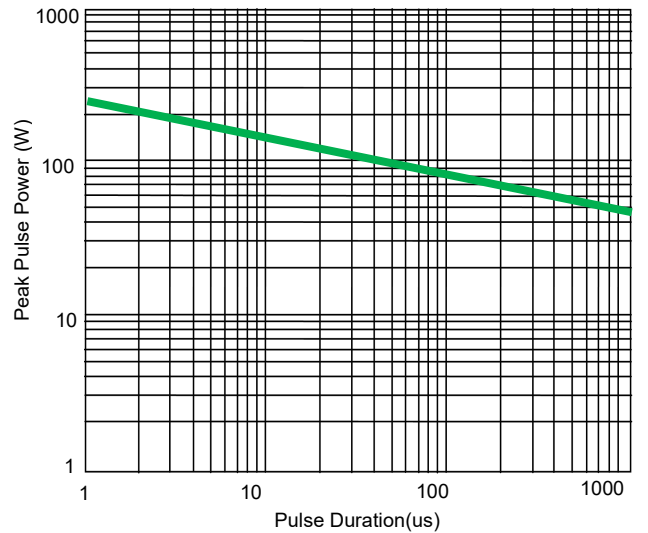
Fig 6. Non-Repertive Peak Pulse Power vs. Pulse time
