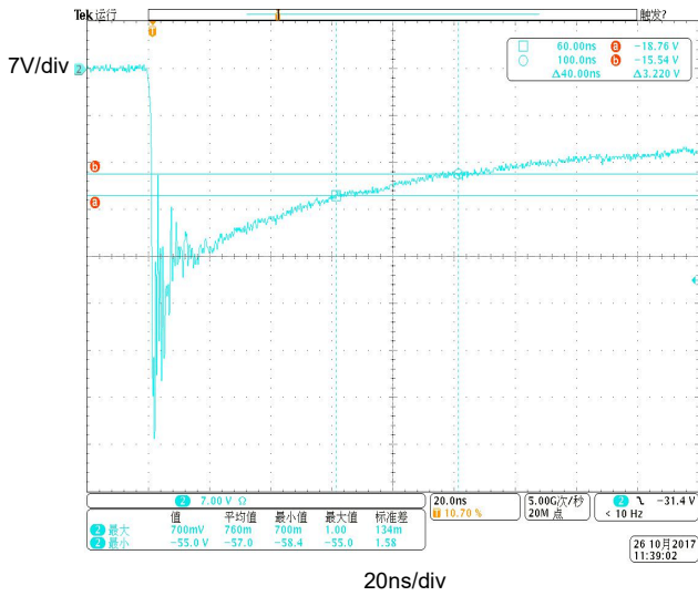
Fig 9. ESD clamping voltage (IEC61000-4-2-8KV contact)
