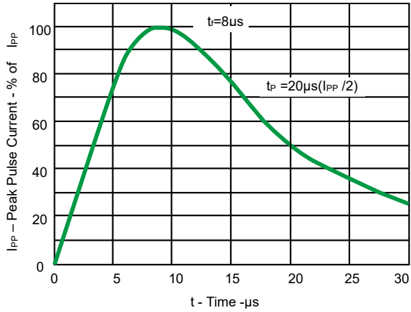
Fig 1. Pulse Waveform
