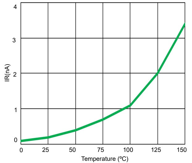
Fig 5. Typical Leakage Current vs. Temperature
