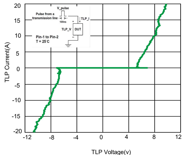
Fig 6. TLP Measurement
