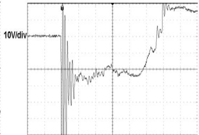
Fig 8. ESD clamping voltage (IEC61000-4-2-8KV contact)
