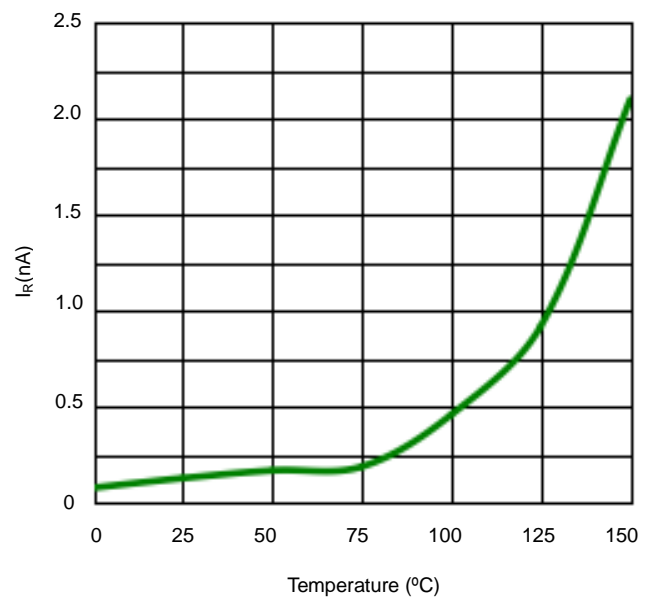
Fig 6. Typical Leakage Current vs. Temperature
