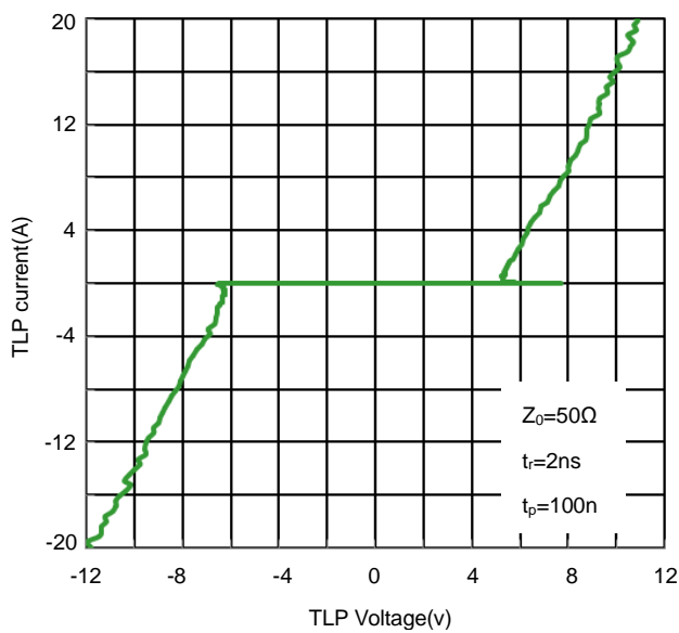
Fig 5. TLP Measurement
