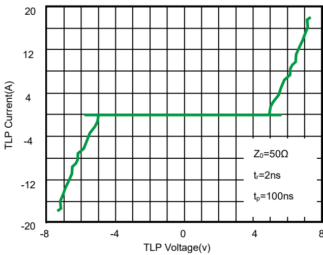
Fig 3. TLP Measurement
