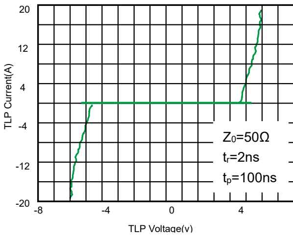
Fig 3. TLP Measurement
