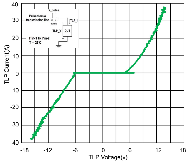
Fig 4. TLP Measurement
