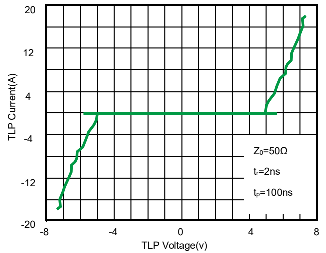
Fig 4. TLP Measurement
