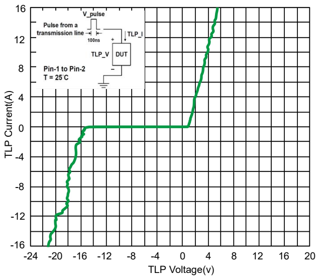
Fig 5. TLP Measurement
