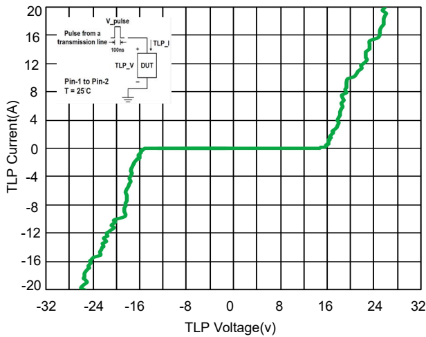
Fig 3. TLP Measurement
