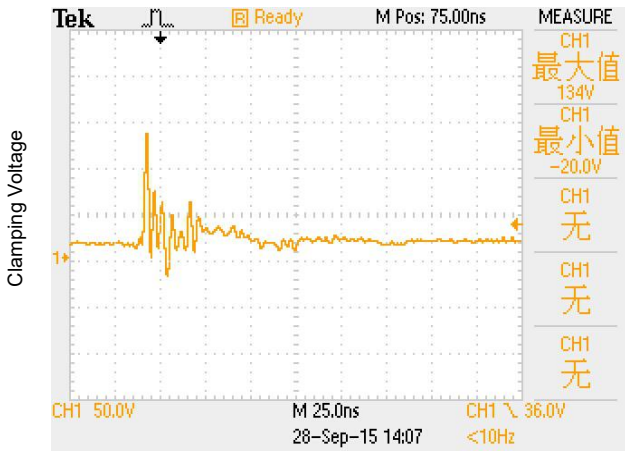
ESD clamping
