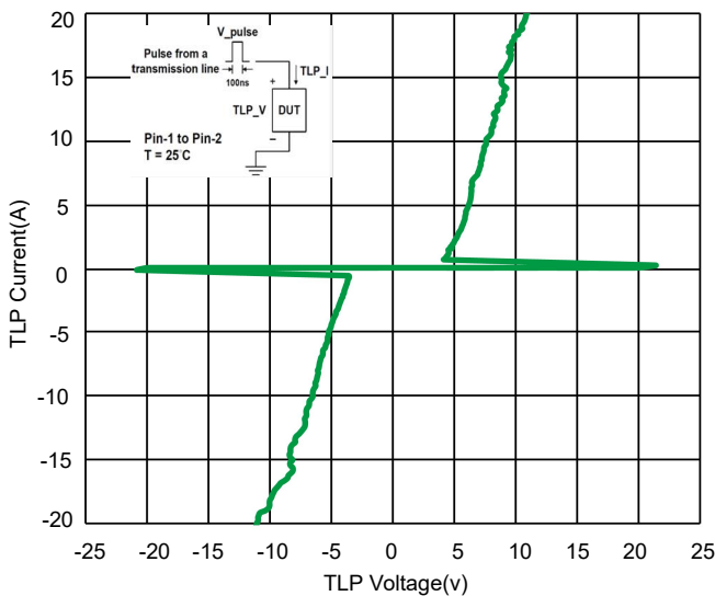
Fig 5. TLP Measurement
