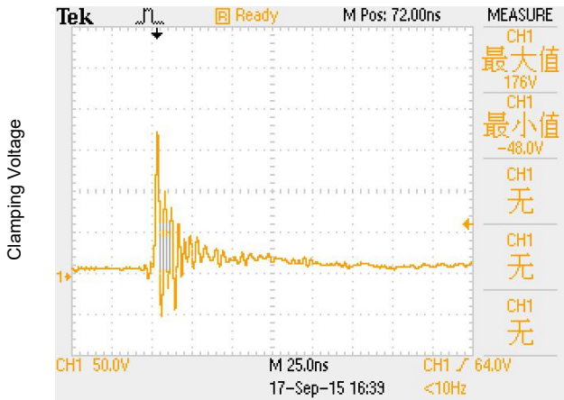
ESD clamping
