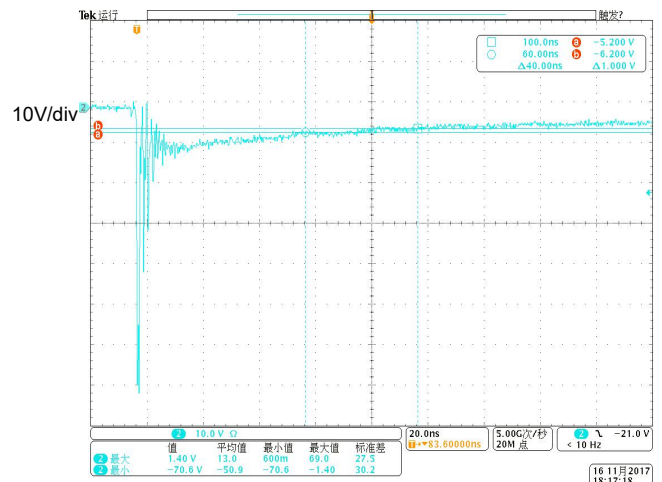
20ns/div Fig 8. ESD clamping voltage (IEC61000-4-2-8KV contact)
