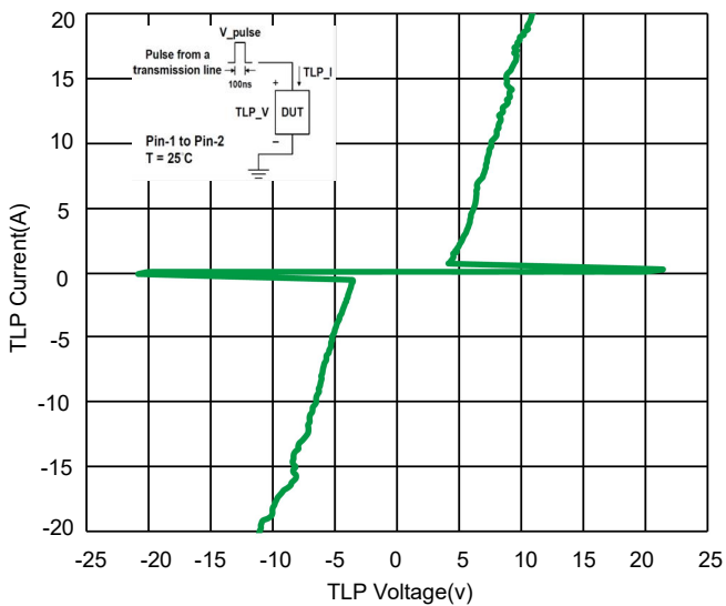
Fig 5. TLP Measurement
