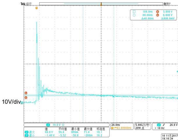
20ns/div Fig 7. ESD clamping voltage (IEC61000-4-2 +8KV contact)
