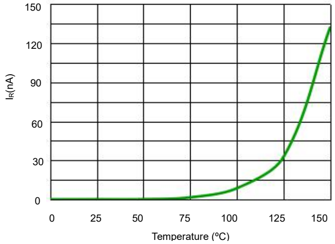
Fig 2. Typical Leakage Current vs. Temperature
