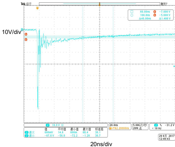
20ns/div Fig 7. ESD clamping voltage (IEC61000-4-2-8KV contact)
