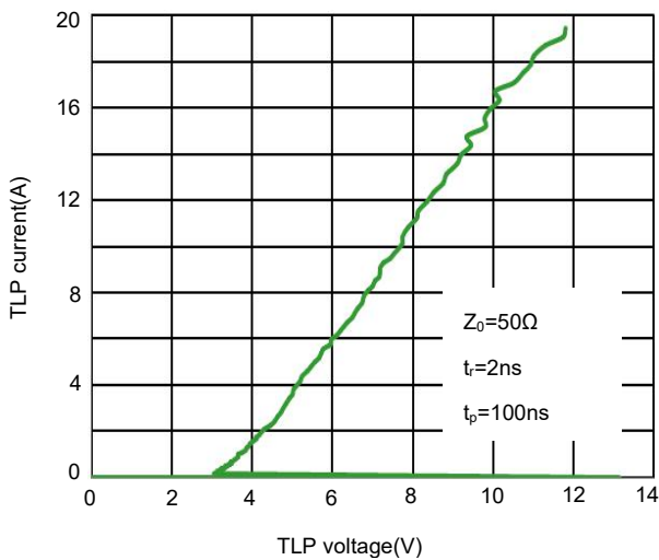
Fig 5 TLP Measurement
