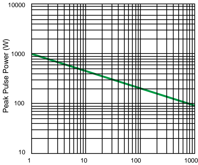
Fig 3. Non Repetitive Peak Pulse Power vs. Pulse time
