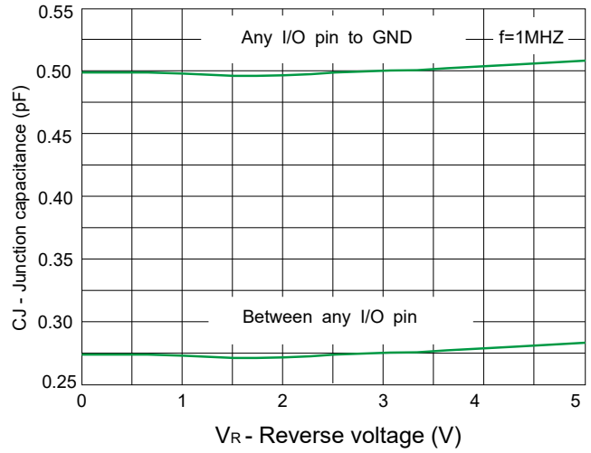
Fig 4 . Capacitance vs. Revers voltage
