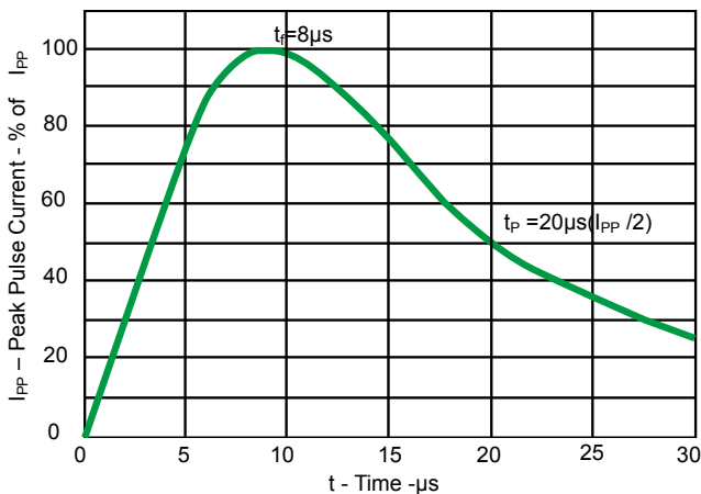
Fig 1.Pulse Waveform
