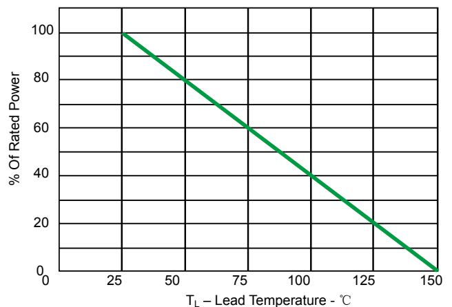
Fig 2.Power Derating Curve
